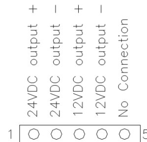
Output connectors
