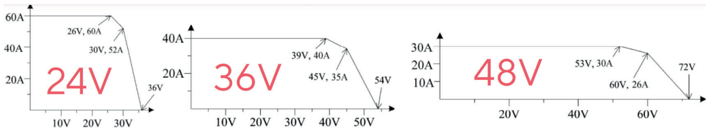
Nominal output voltage / current characteristics 1600W models
