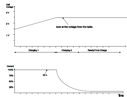
Constant Voltage Charger
