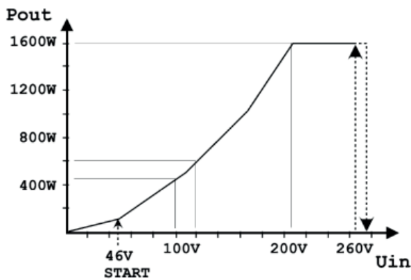
Output power / input voltage derating curve
