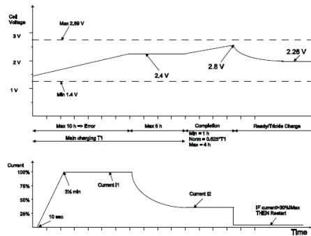
Unsealed Battery
