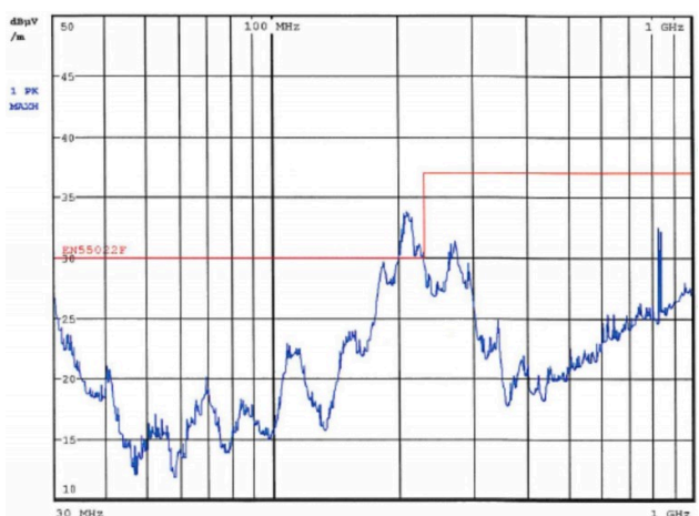
Typical radiated emissions at 115 V AC 60 Hz
