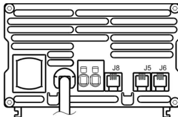
Rear panel
