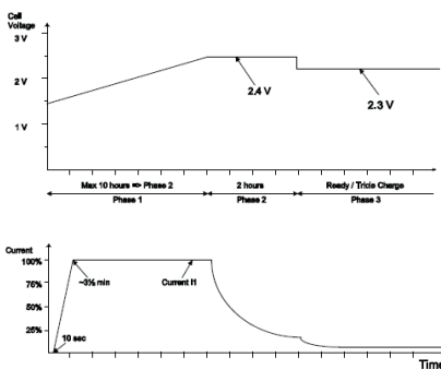
Extended Charger
