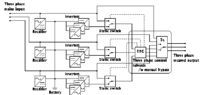
3-phase system Same inverter modules
