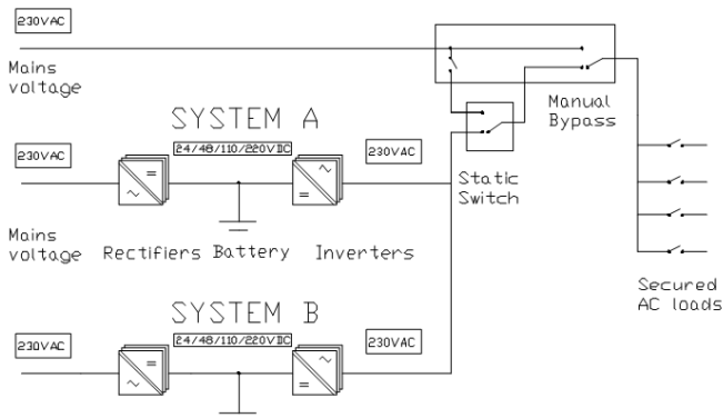
Dual Redundant Double battery system
