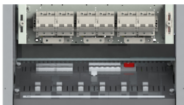
Type B Battery MCBs in Battery connection panel max 250A, 2-pole, 1-3pcs
