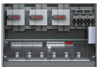
Type D Battery Switch fuses in Battery connection panel max 125A, 2-pole, 1-3pcs
