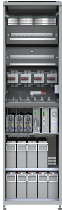
OPUS HE 110-6.0 OC2066 110VDC 18.5A – 111A Inverter AC power up to 3.6kW 2 x Switch Fuse 125A batt fuses Battery & distribution space Inverter system option
