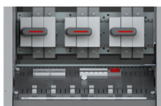
Type E Battery Switch fuses in Battery connection panel max 250A, 2-pole, 1-3pcs
