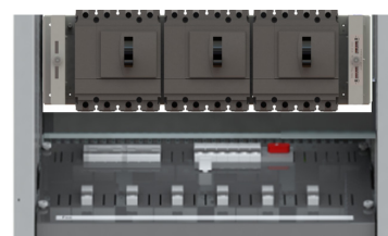
Type C Battery MCCBs in Battery connection panel max 460A, 2-pole, 1-3pcs
