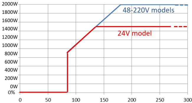
Output power vs. AC input voltage
